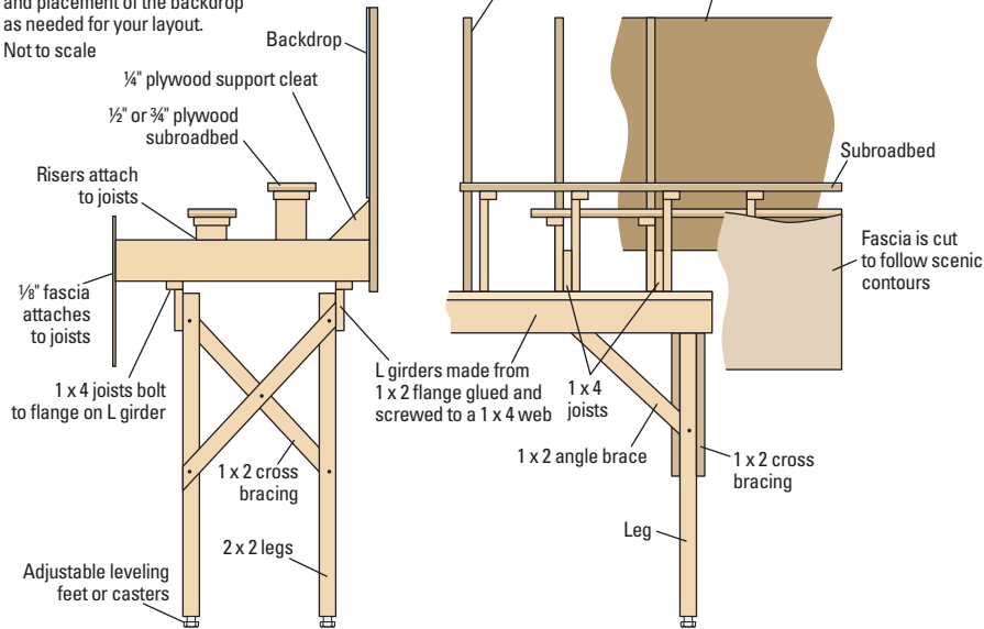
End view
