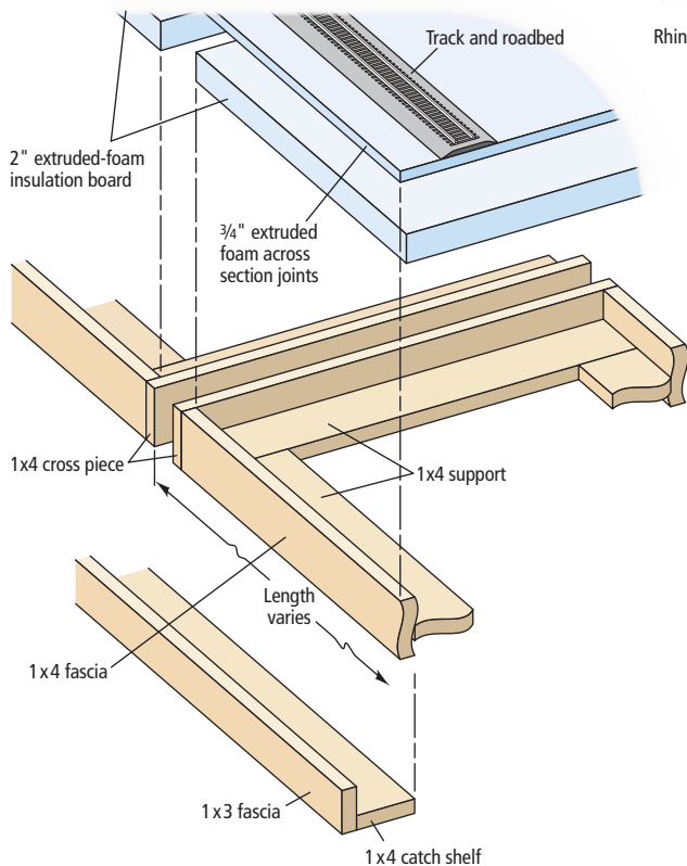
Layout benchwork
