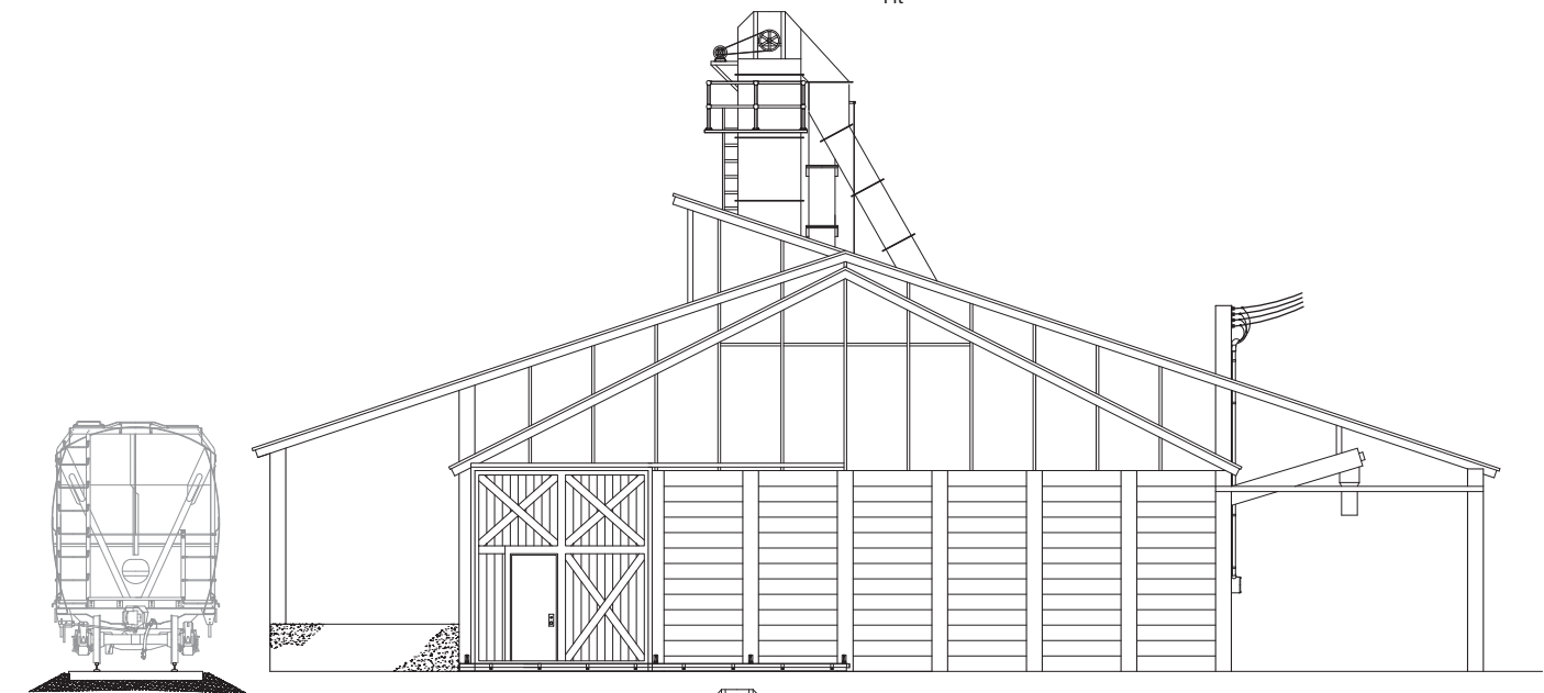
Section at elevator
