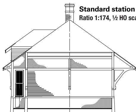
Baggage room end elevation
