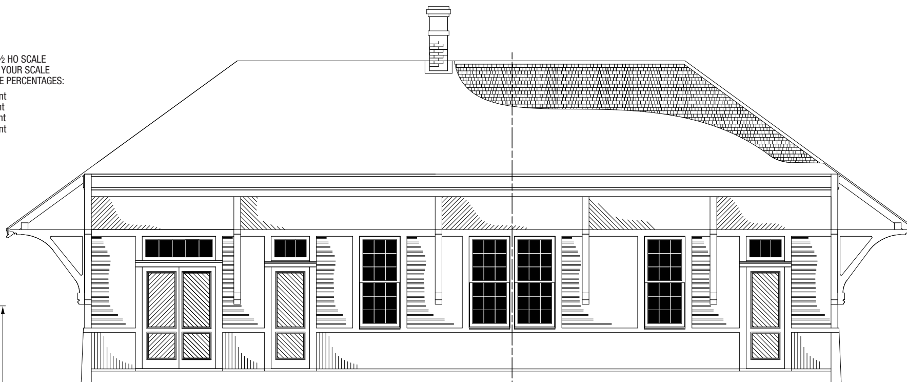
Rear elevation
