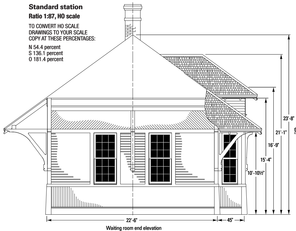
Waiting room end elevation
