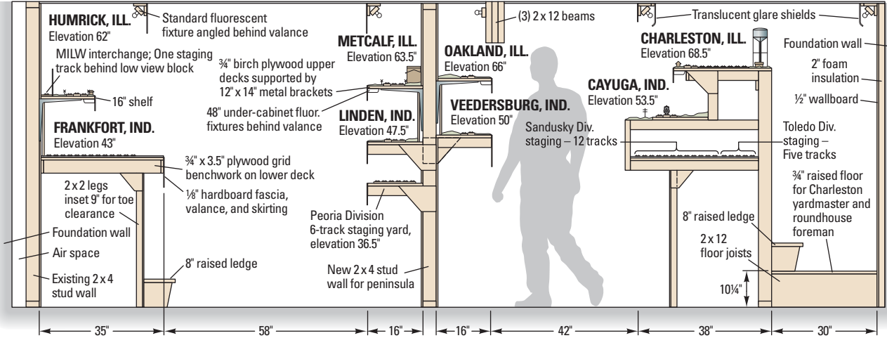
CROSS-SECTION A-A
