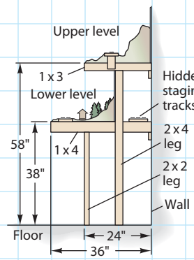
Benchwork cross section
