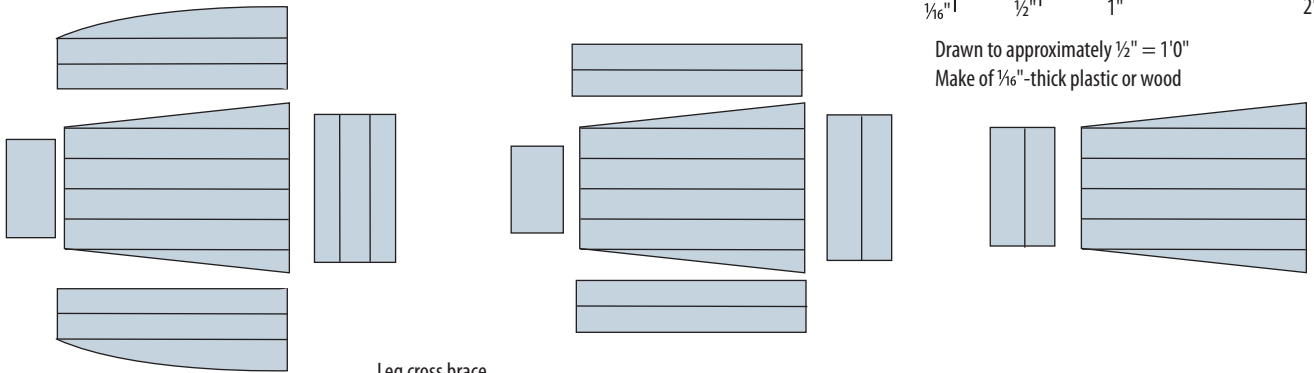
Frame and handles 2 required
